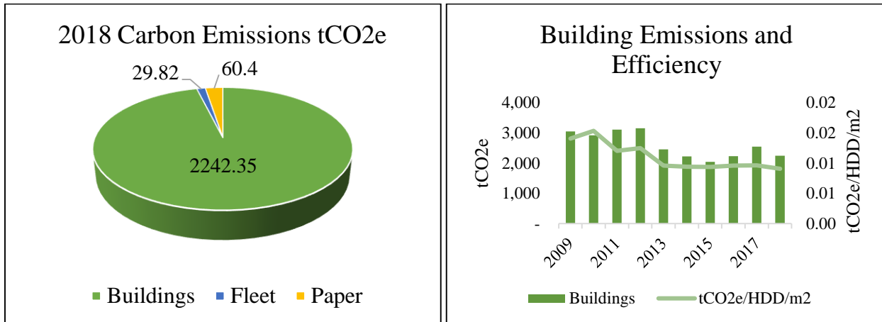
Figure 1: 2018 Carbon emissions by source.
