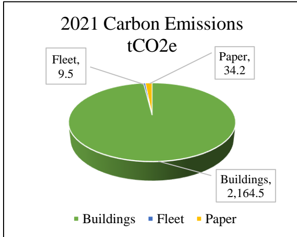
Figure 1: 2021 Carbon emissions by source.
